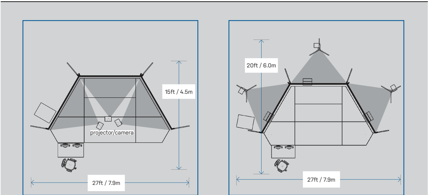
FRONT PROJECTION
