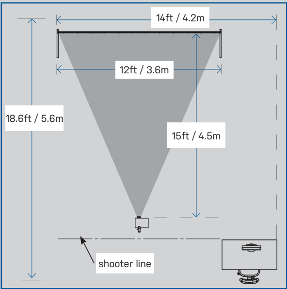
FRONT PROJECTION
